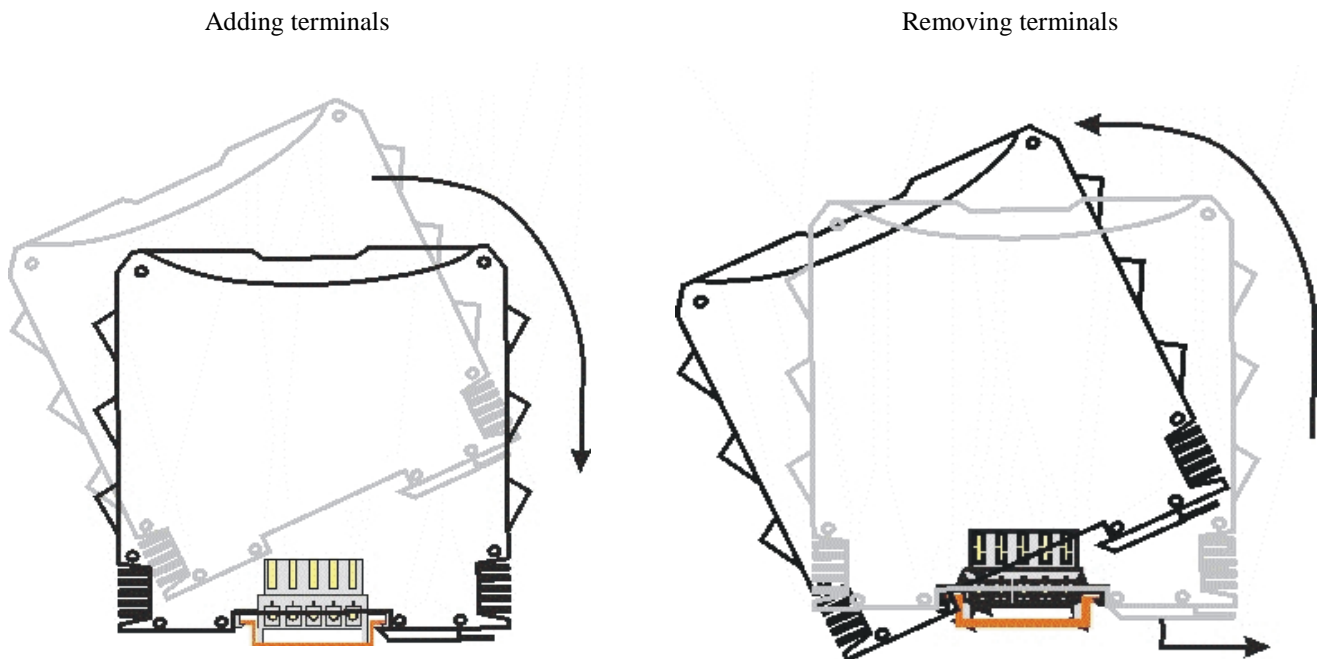
Figure 3 Insertion and removal of a terminal
