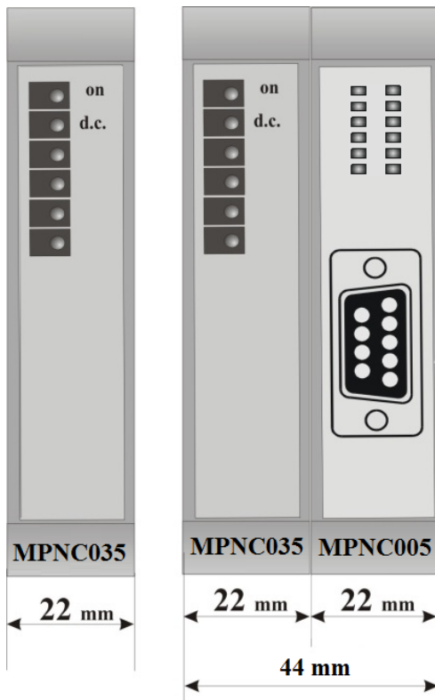
Figure 1 Dimensions
