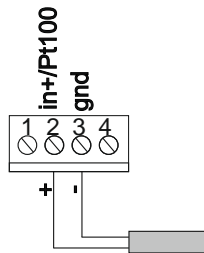
Thermocoupling input connection
