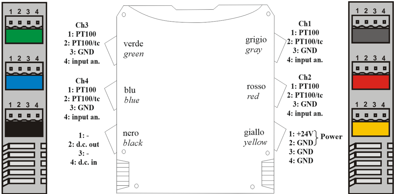
Fig 8: Signals connection
