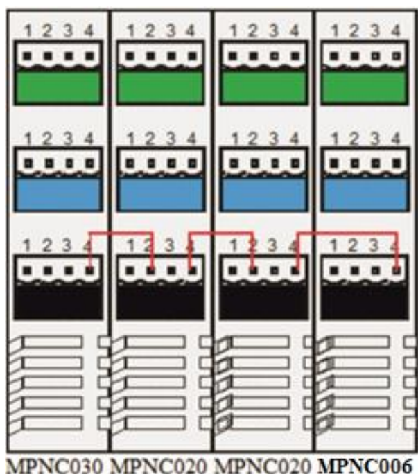
Fig 6: Collegamento MPNC006
